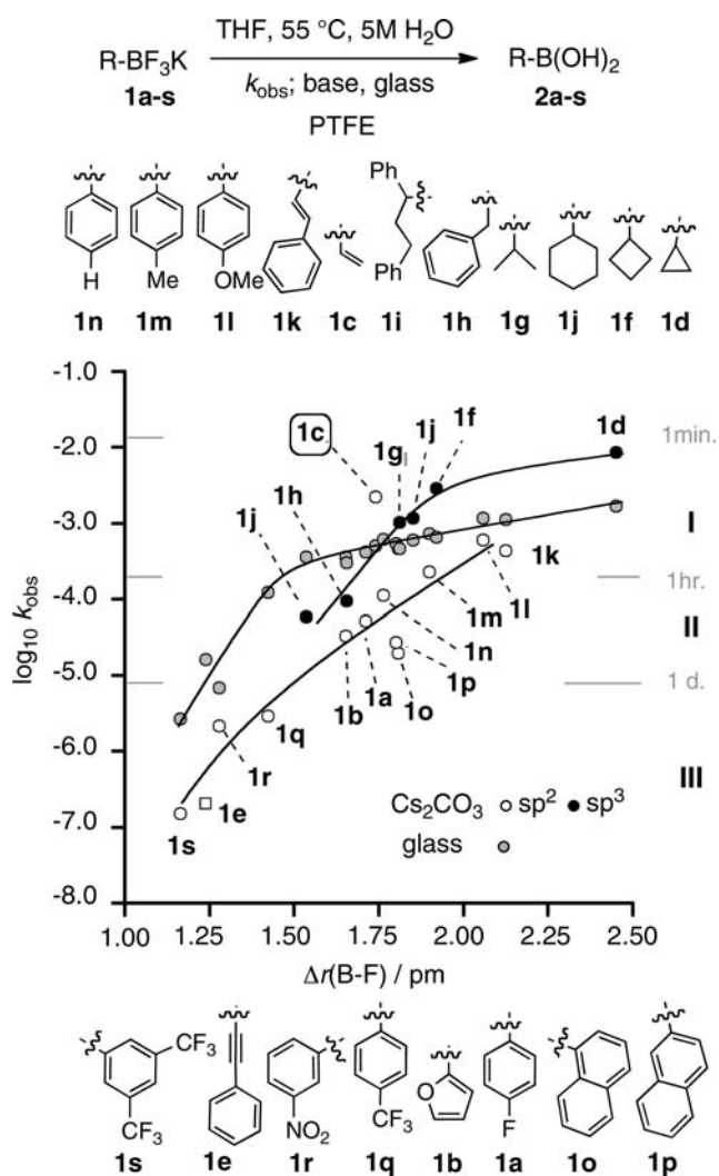
Figure 9. Bond elongation ( \Delta r(\text{B–F}) ) 39 in RBF 2 (3a–s) versus \log_{10} k_{\text{obs}} \text{ (s}^{-1}\text{)} for hydrolysis of 1a–s (8 mM) mediated by glass powder and by Cs 2 CO 3 in 10/1 (v/v) of THF/water (5 M H 2 O) at 55 °C in a PTFE vessel with 500 rpm magnetic stirring. Lines through data are a solely a guide to the eye. Reagents classed by t_{0.5} in base (I, \leq 1 \text{ h} ; II 1 h–24 h; III \geq 1 \text{ day} ).
