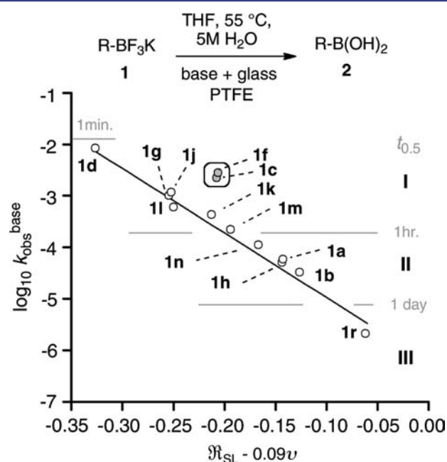
Figure 10. Rates of base-mediated hydrolysis of 1 versus combined resonance ( \mathcal{R}_{\text{SL}} ) 45 and steric ( \nu ) 46 parameters. Vinyl 1c is a mechanistic outlier; see text for discussion. The validity of the \mathcal{R}_{\text{SL}} value for cyclobutyl 1f 43 is uncertain. Reagents have been classed by t_{0.5} in base (I, \leq 1 h; II 1–24 h; III \geq 1 day).
