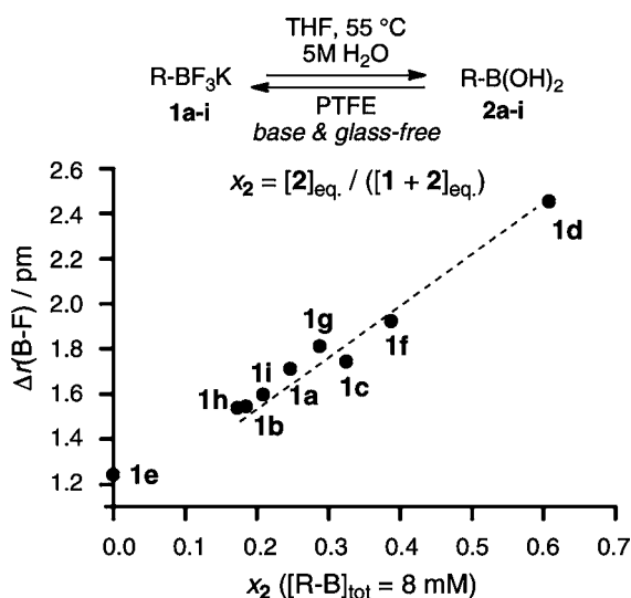
Figure 8. Variation in B–F bond length ( \Delta r(\text{B–F}) , by DFT) in RBF 2 (3a–i) with hydrolytic equilibrium ( x_2 ) 35 for RBF 3 K (1a–i) → RB(OH) 2 (2a–i) at [\text{RB}]_{\text{TOT}} = 8 \text{ mM} ; x_2 for 1e was not determined. 37 \Delta r(\text{B–F}) = 0.0018 \ln K + 0.0474 .
